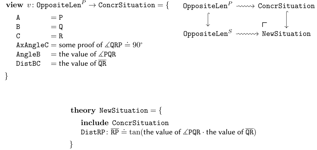
Figure 4: The NewSituation Theory as a result of a pushout
