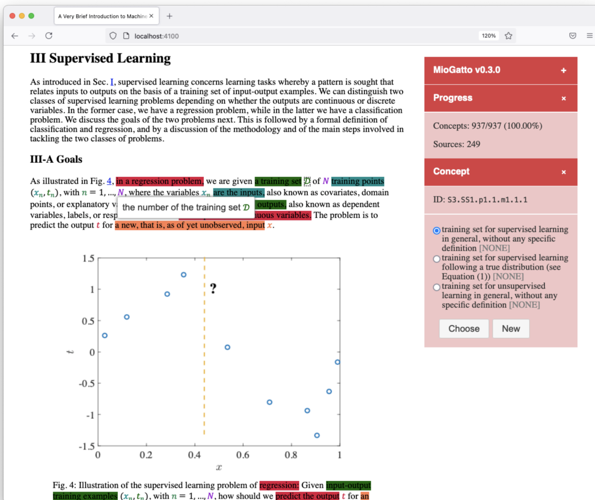
Figure 2: The screen of MioGatto. This is a captured image of annotating an arXiv paper in the field of machine learning [Sim18]. The basic annotation operations, such as selecting the math concept that each identifier refers to, are performed in a sidebar on the right. Each occurrence of an identifier is colored according to the annotated math concept. In other words, identifiers with the same color have a coreference relation. Grounding sources are also highlighted in colors that correspond to math concepts associated with them. When the mouse is over an annotated occurrence, the tooltip with the description of the corresponding math concept is shown.
